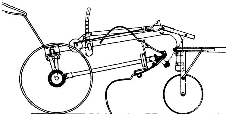
FIG. 2.—Diagram of Blackstone's Swath Turner, No. 3676.
