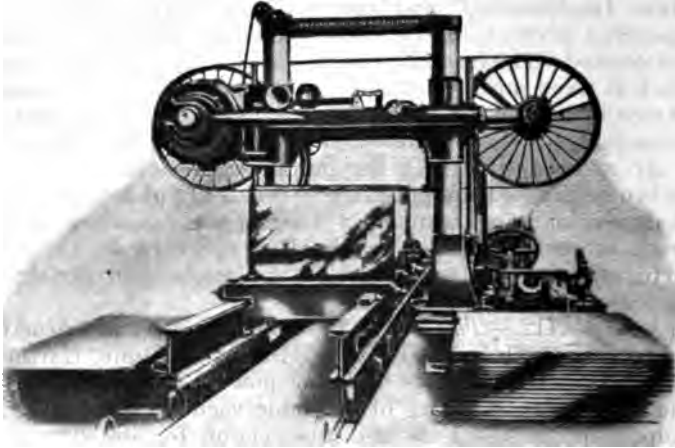
FIG. 3.—Horizontal Log Band Saw.
